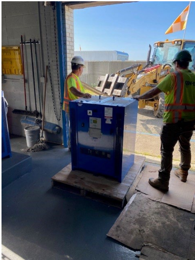
Constant Current Regulator (CCRs) Installation in the electrical vault
